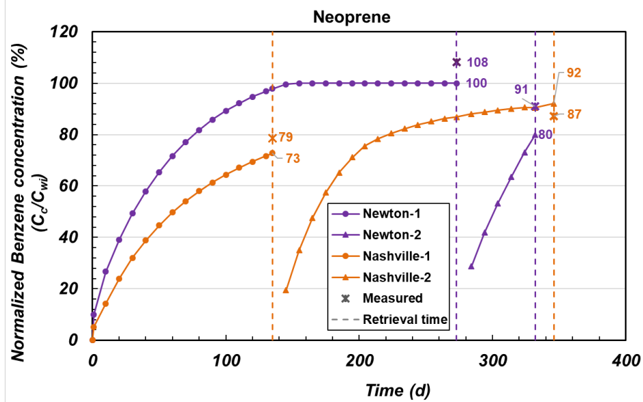
(a) Neoprene
