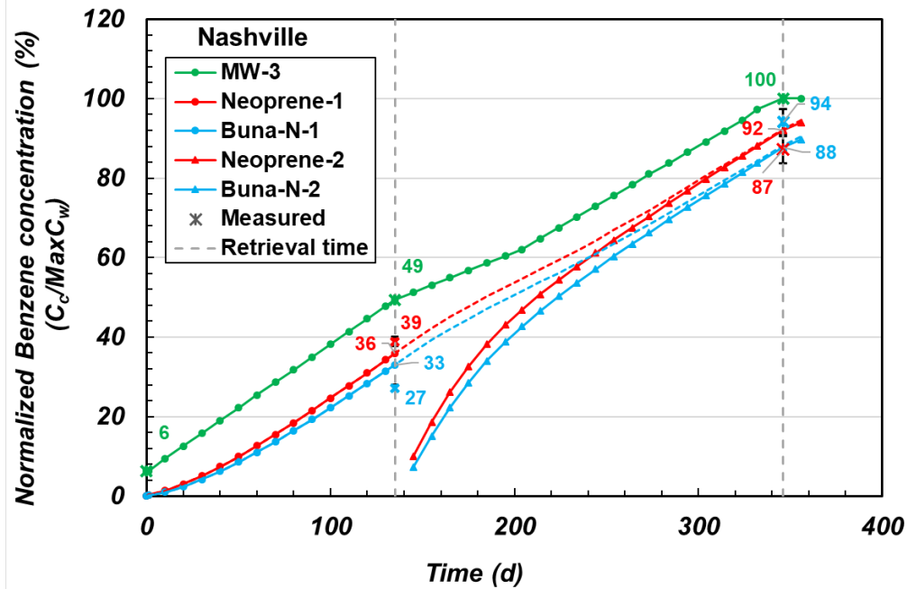
(a) Nashville site
