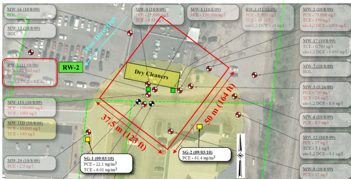
Figure B3 Durham site map and model domain (After URS 2015).
